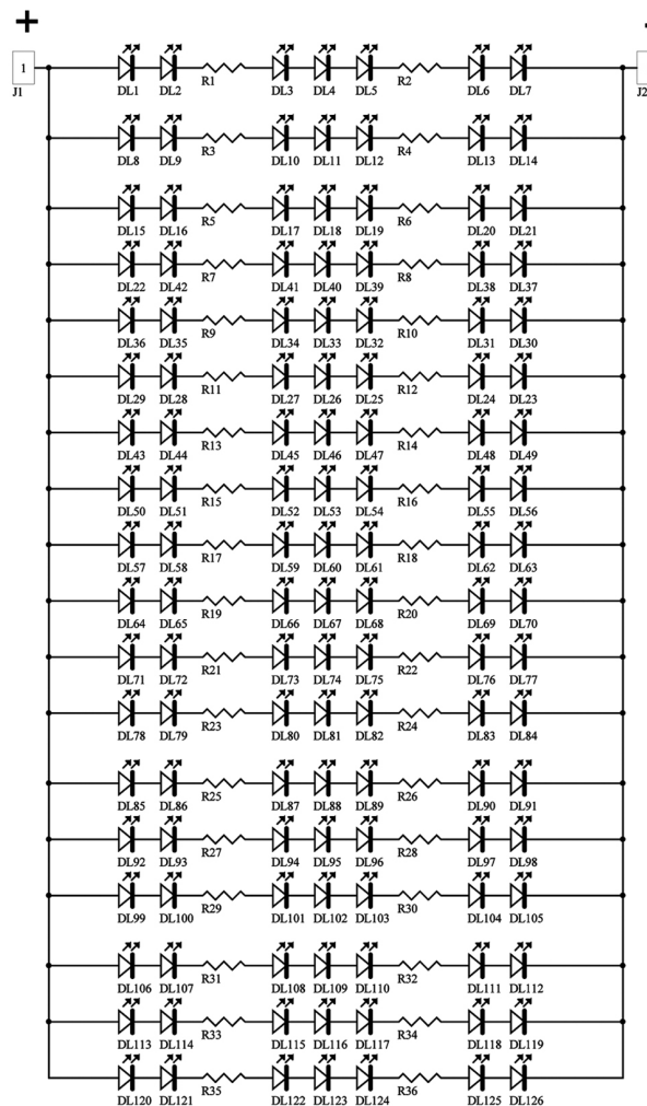
SCHEMA COLLEGAMENTO WIRING DIAGRAM
